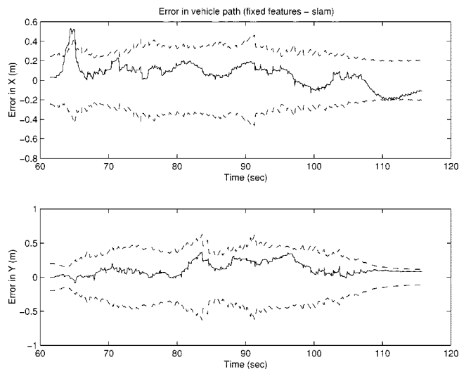
Fig. 8. Actual error in vehicle location estimate in x and y (solid line), together with 95% confidence bounds (dotted lines) derived from estimated location errors. The reduction in the estimated location errors around 110 s is due to the vehicle slowing down and stopping.
